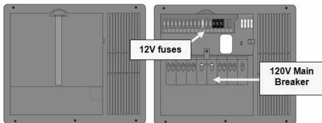
Typical Load Center Panel
