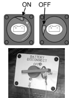
Battery Disconnect Switches
